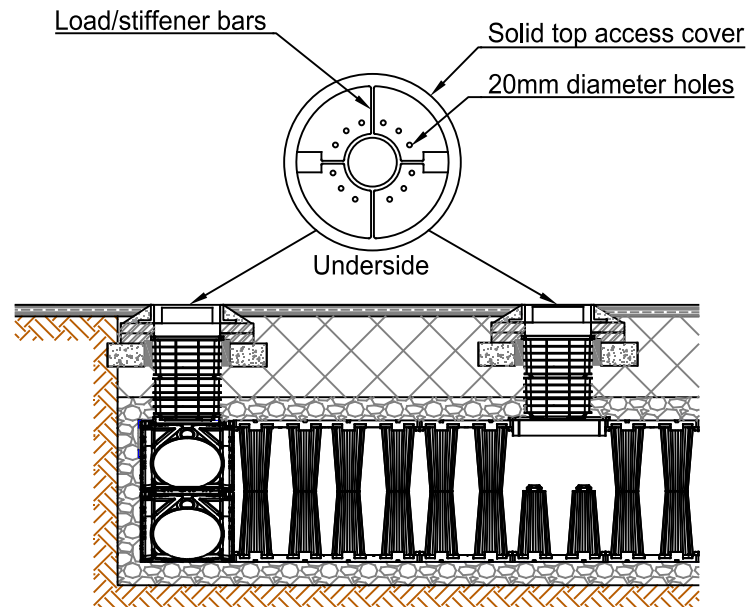
Vent Through Access Cover
