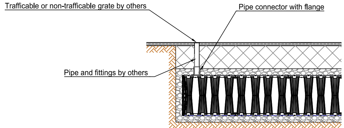
Vertical Vent to Surface
