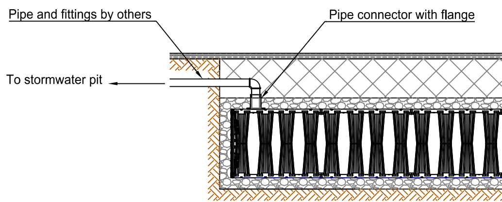
Vertical Vent to Pit
