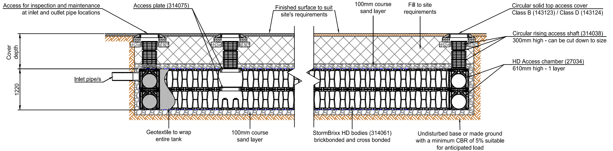
Typical cover depths (1) over the top of ACO StormBrixx HD
