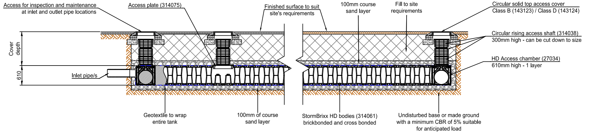
Typical cover depths (1) over the top of ACO StormBrixx HD
